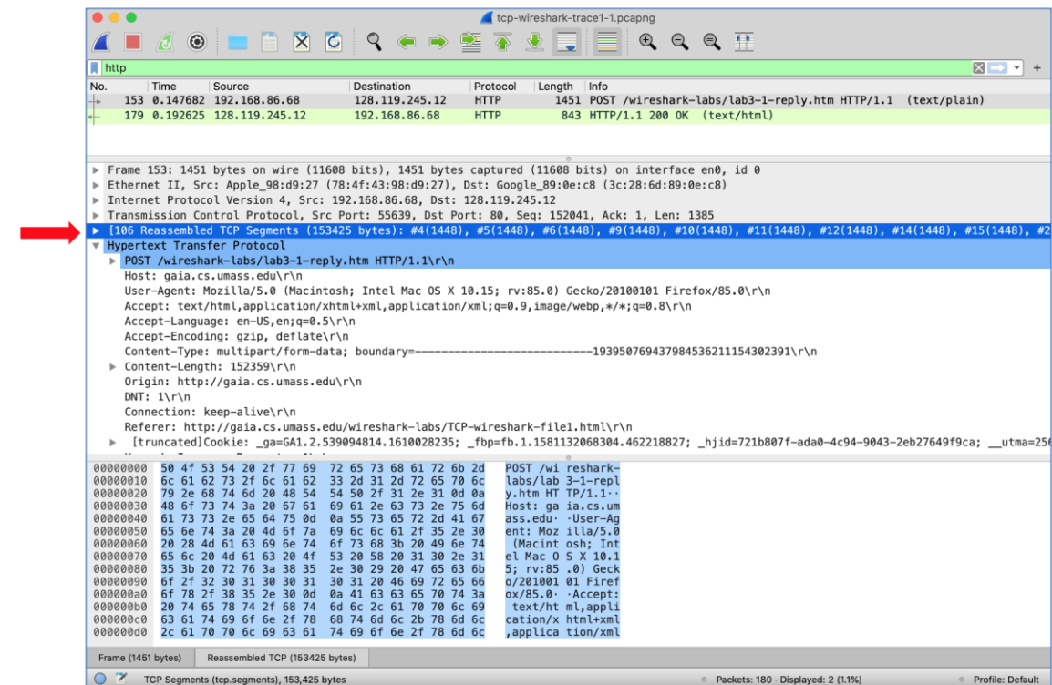
Figure 3: expanding the HTTP POST message that uploaded alice.txt from your computer to gaia.cs.umass.edu
