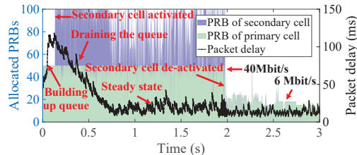
Figure 2: When the offered load of the server exceeds the maximum capacity of the primary cell, cellular network activates a secondary cell for the mobile user to support the high data rate, and deactivates it if the rate drops.
