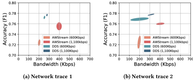
Figure 17: Impact of available bandwidth on performance under re-scaled real network trace.
