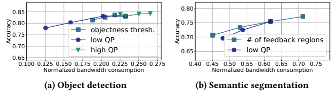
Figure 18: Sensitivity analysis of DDS’s parameters. By varying these parameters, DDS can flexibly adapt itself to reach desirable accuracy for a given bandwidth constraint.
