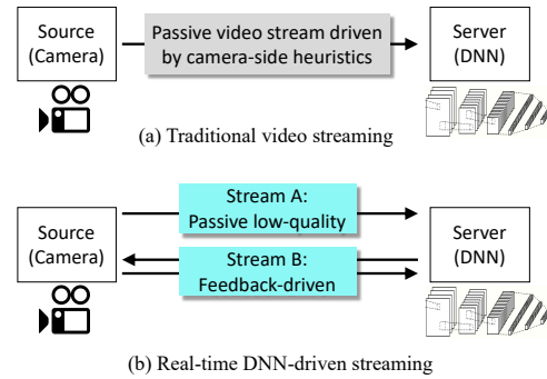
Figure 6: Contrasting the new real-time DNN-driven streaming (iterative) with traditional video streaming in video analytics.
